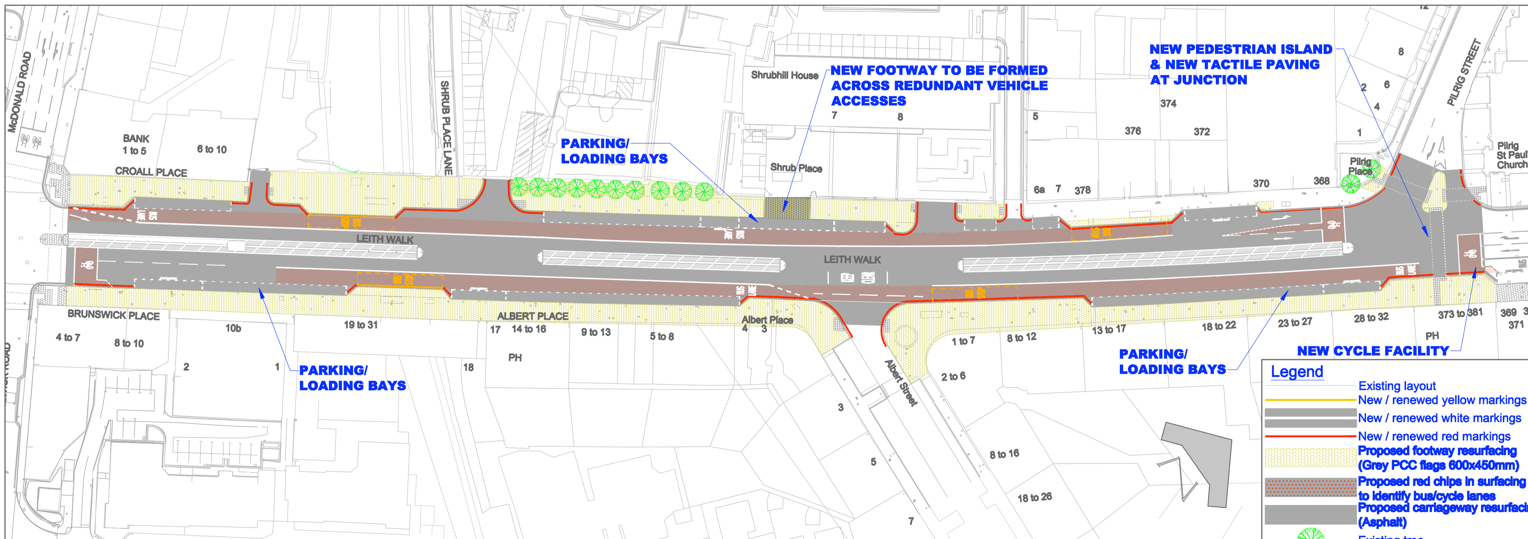
PROPOSED LEITH WALK IMPROVEMENTS BETWEEN McDONALD ROAD AND PILRIG STREET (SECTION 4)
